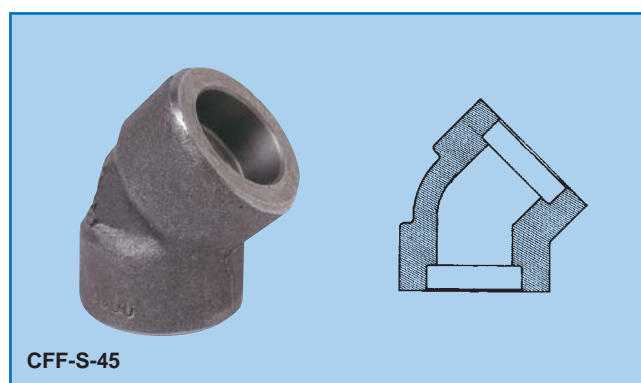
45° SOCKET FEMALE ELBOWS (SW x SW)
